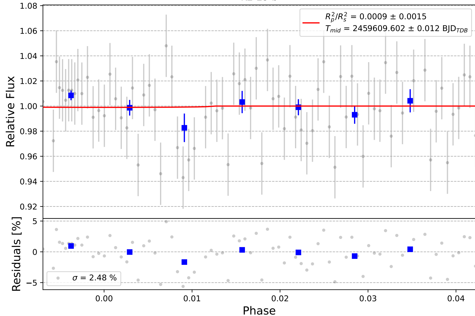
K2-29 b
