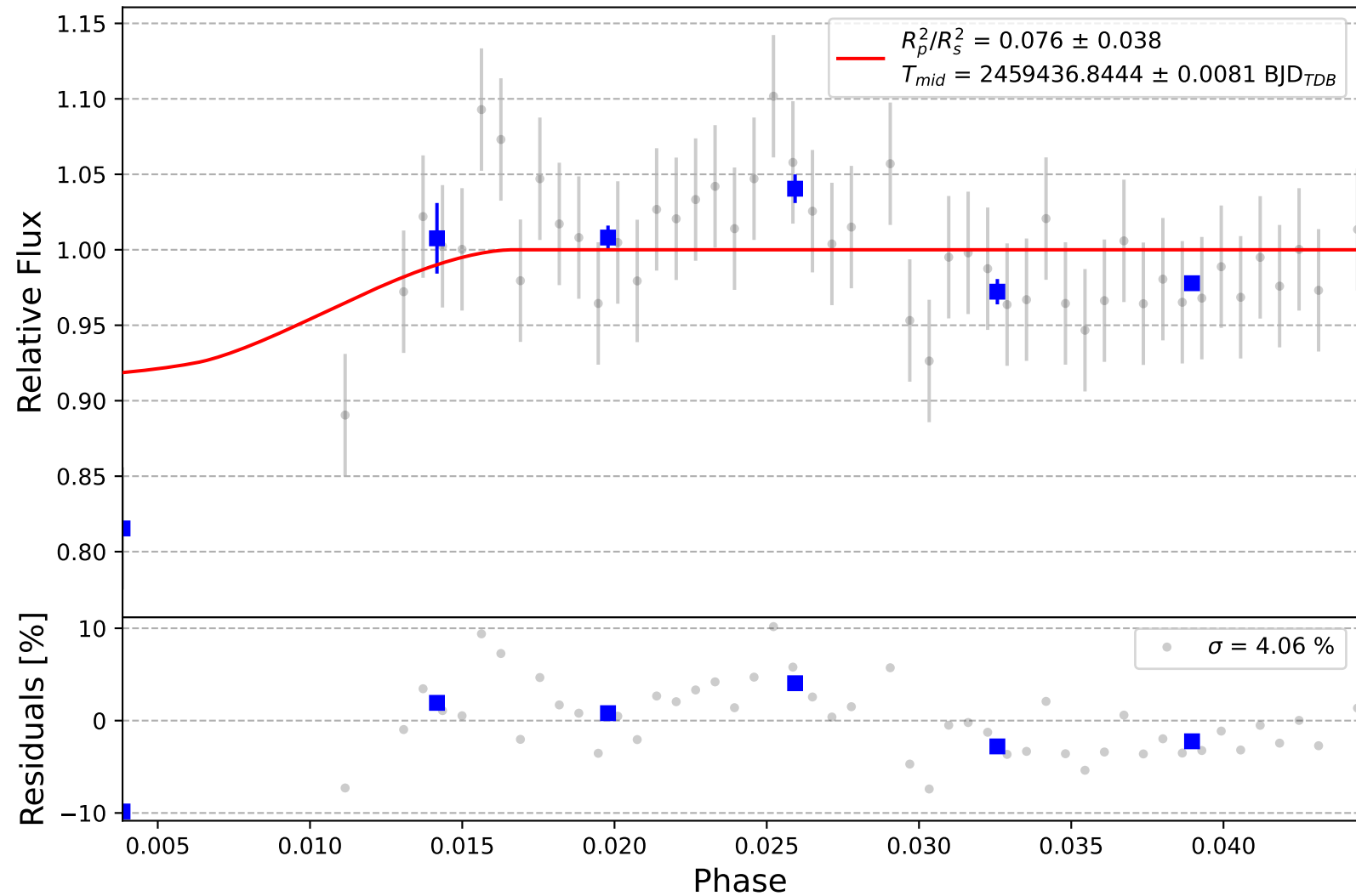
K2-29 b
