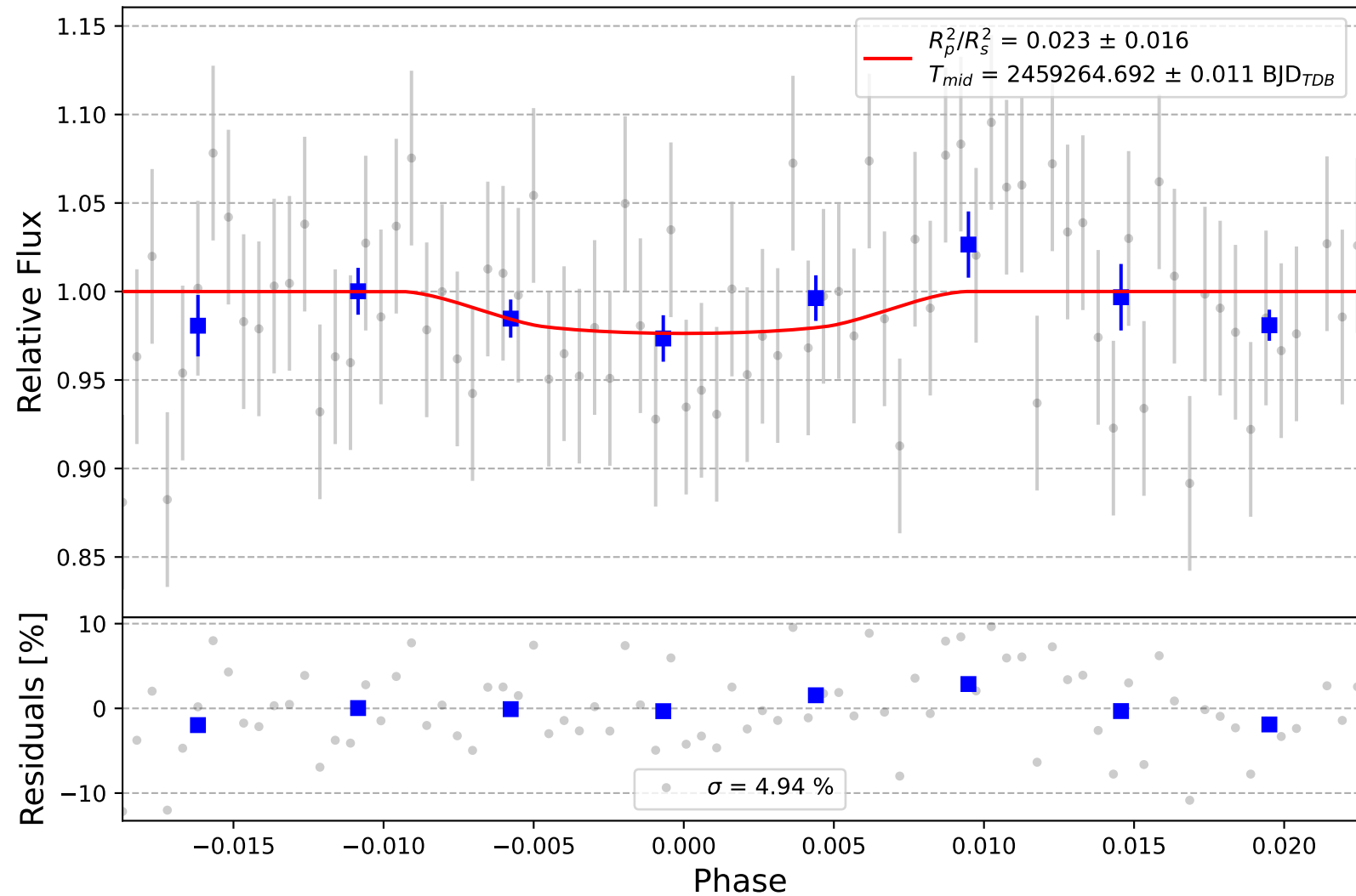
K2-30 b
