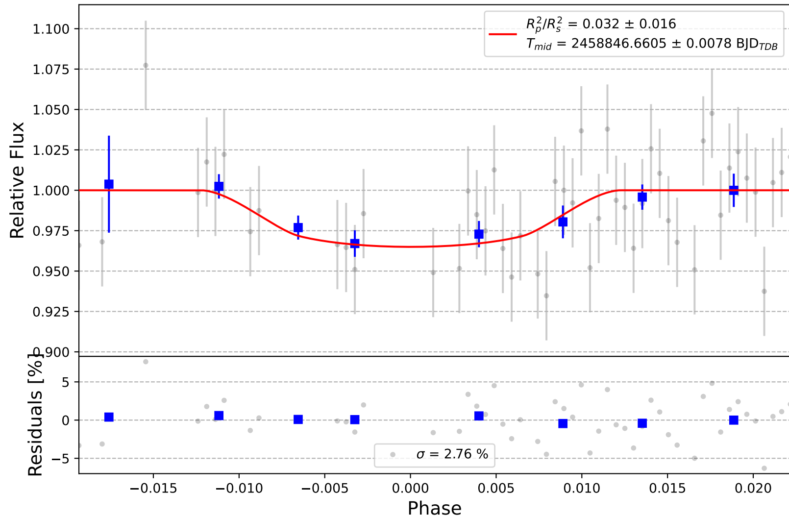
K2-30 b
