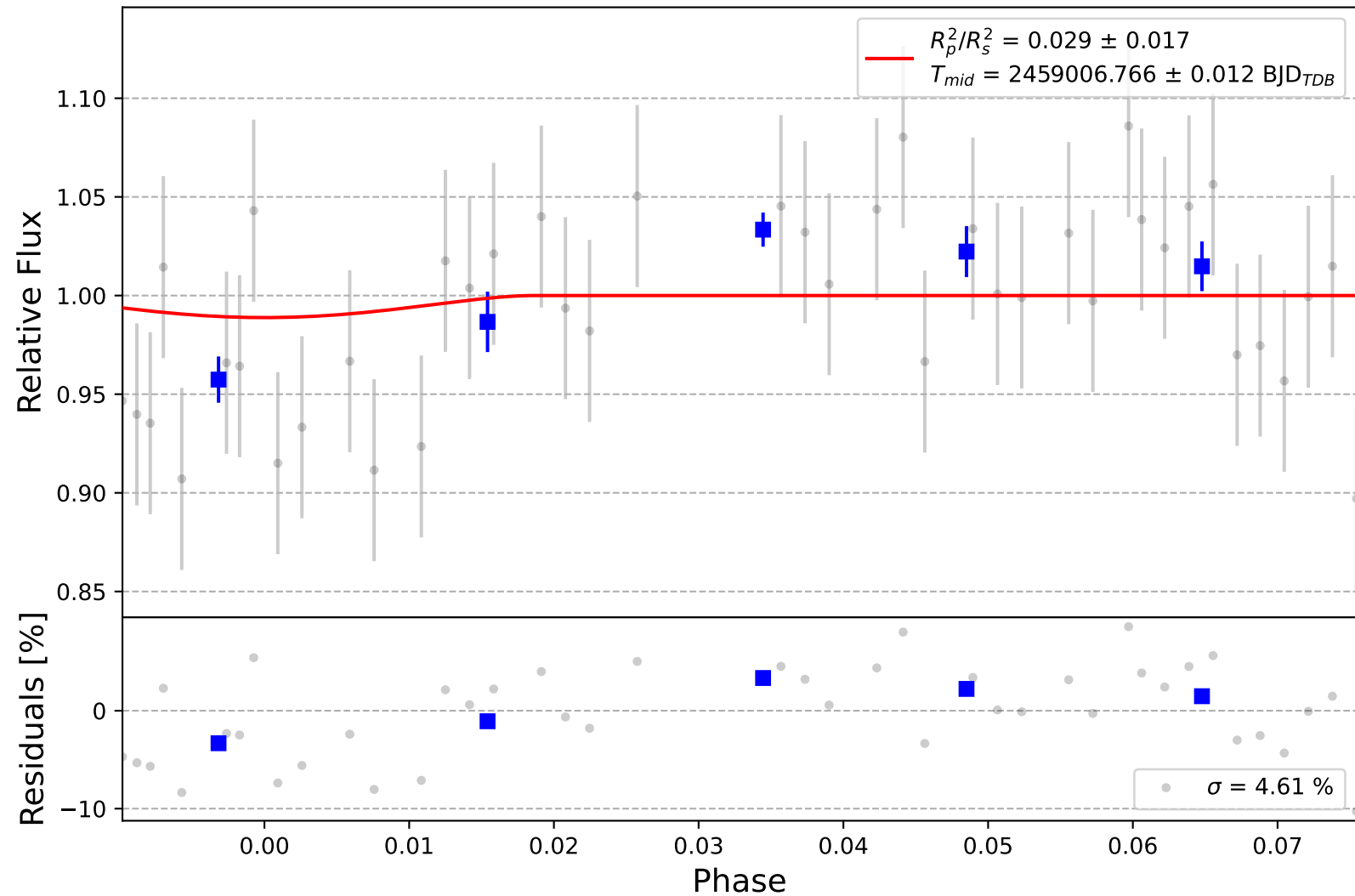
K2-31 b
