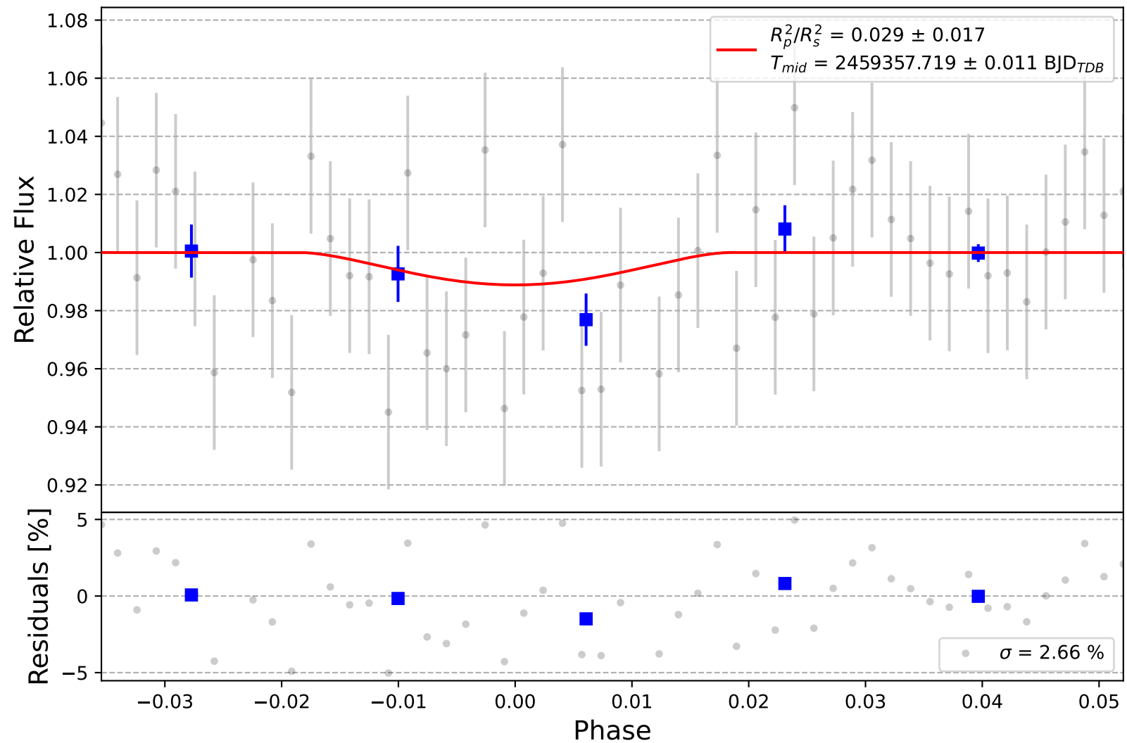
K2-31 b
