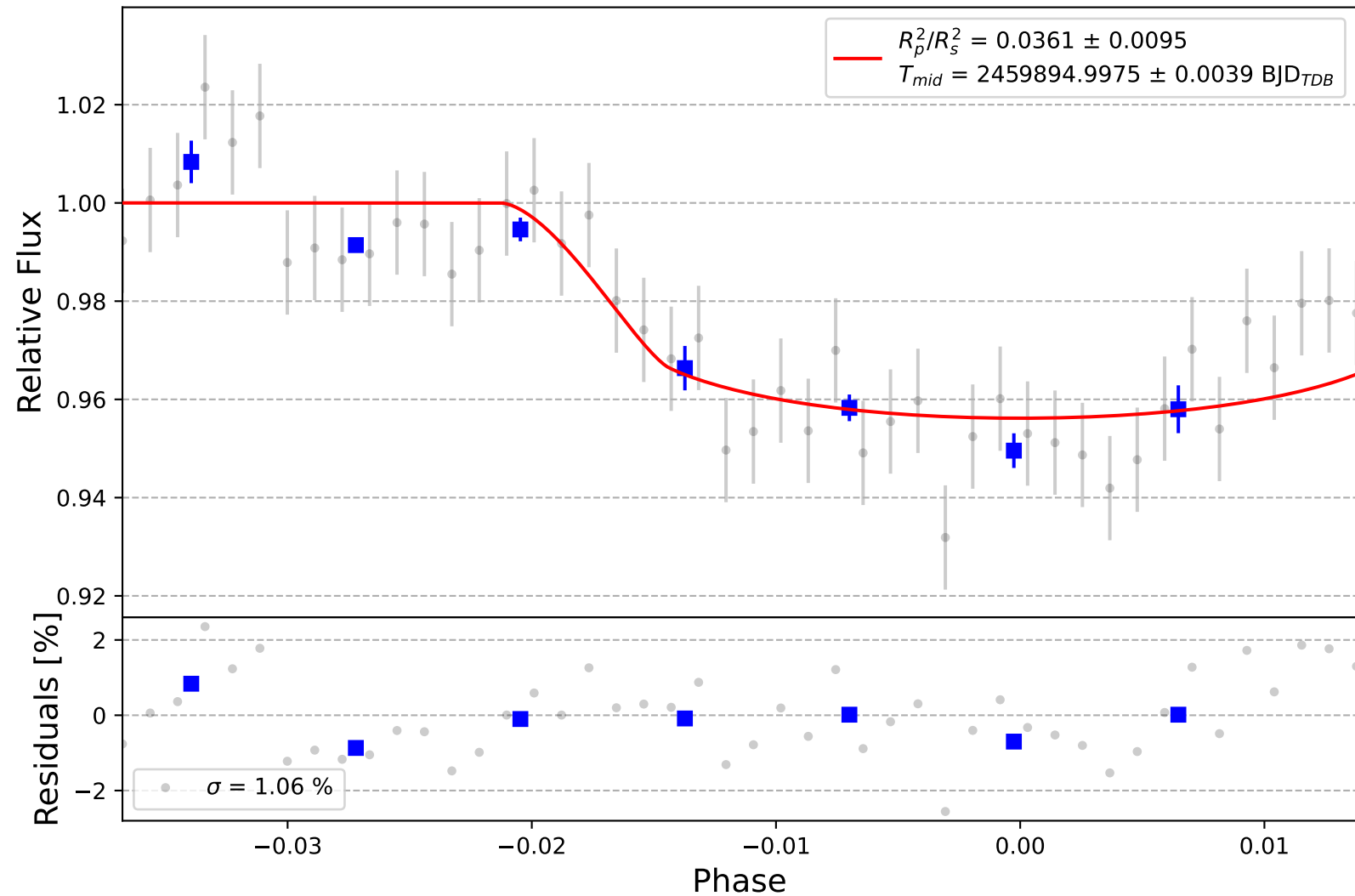
K2-371 b
