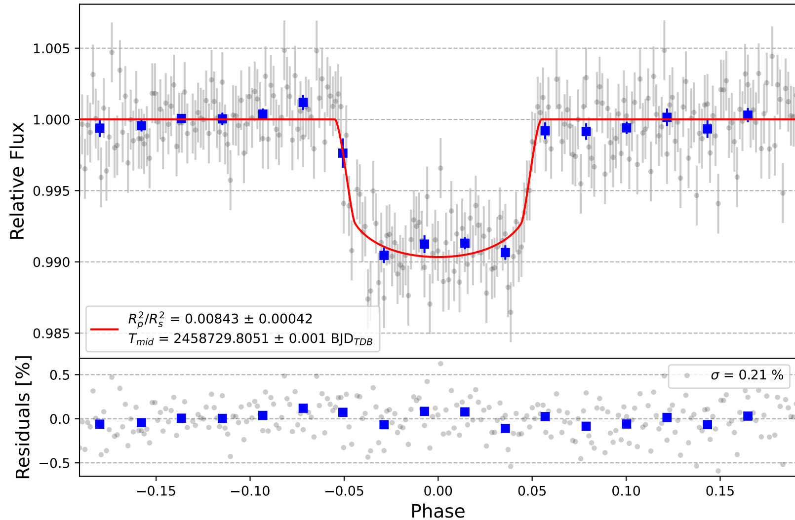
KELT-16 b
