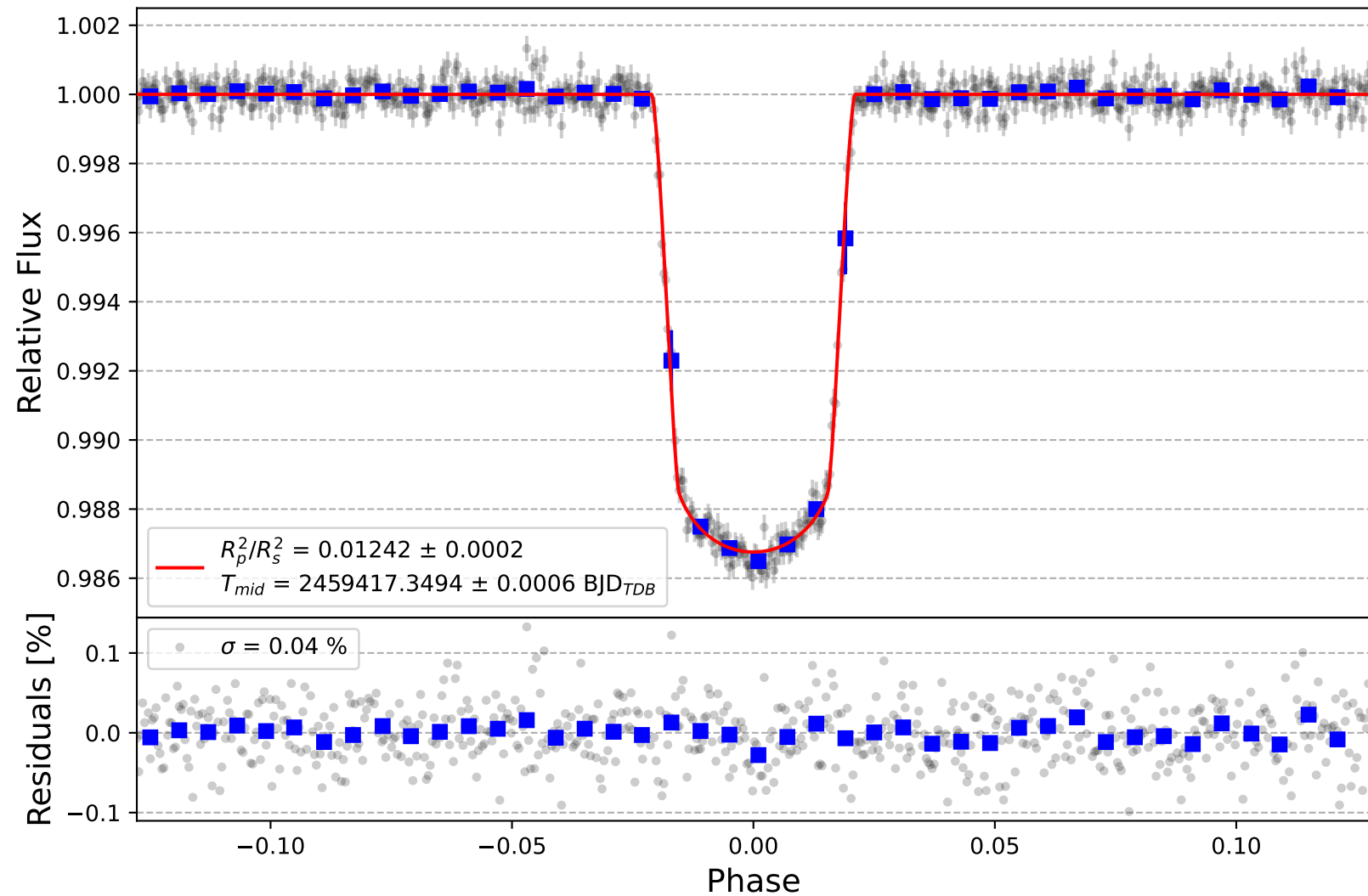
KELT-20 b
