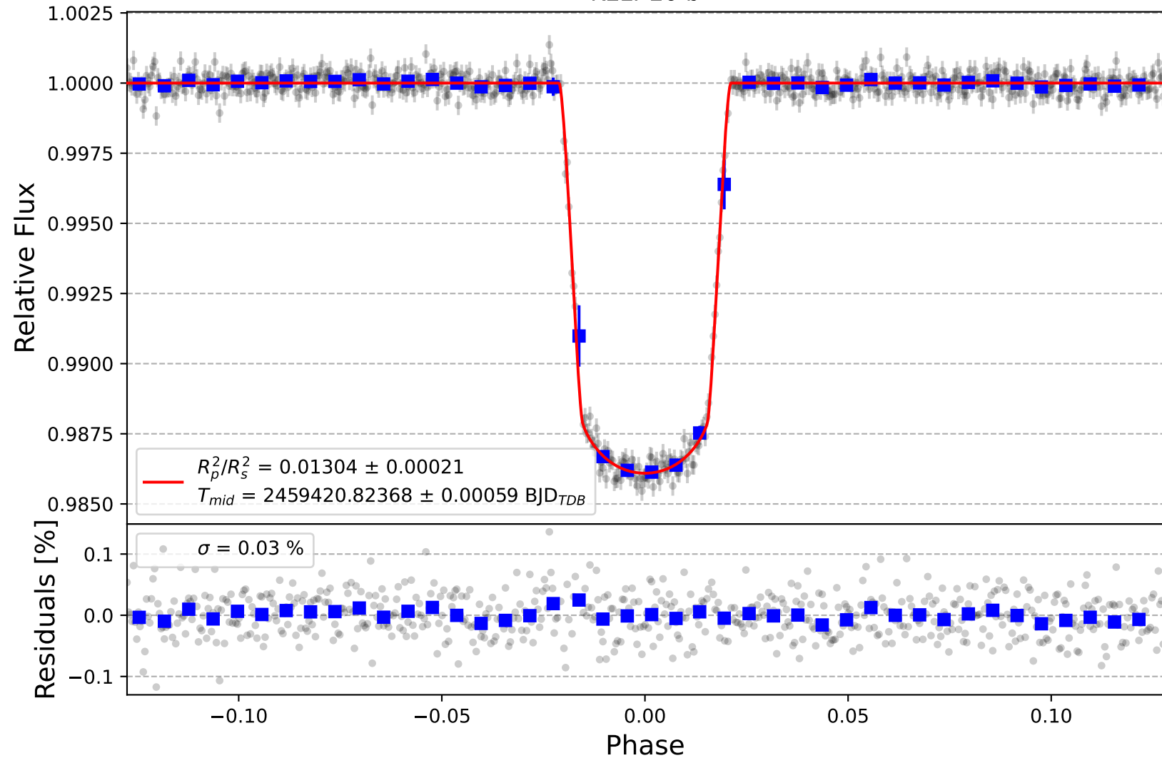
KELT-20 b
