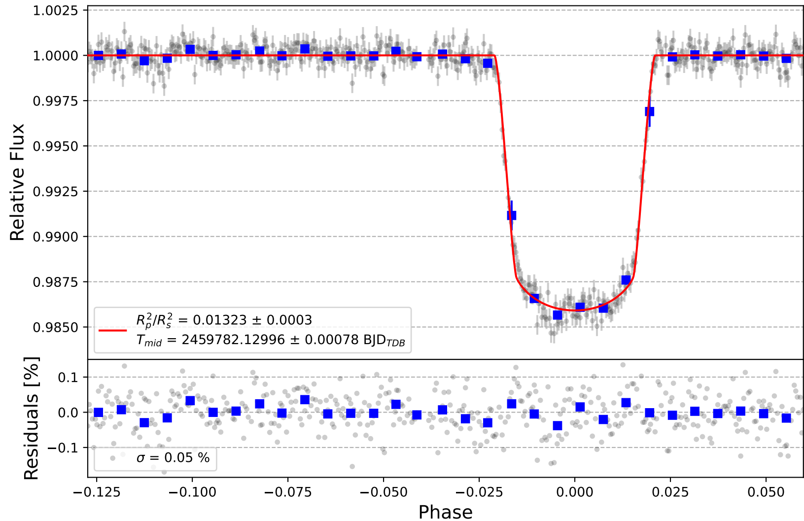
KELT-20 b
