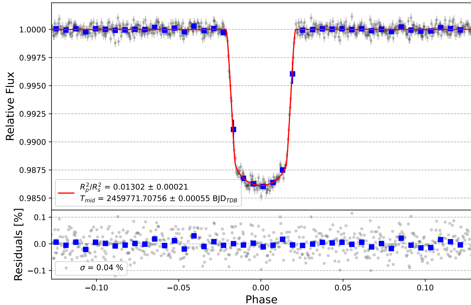
KELT-20 b
