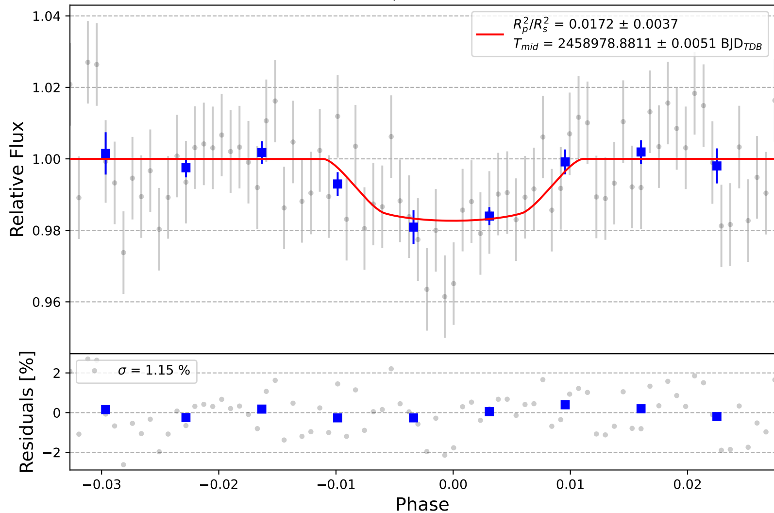
Kepler-426 b
