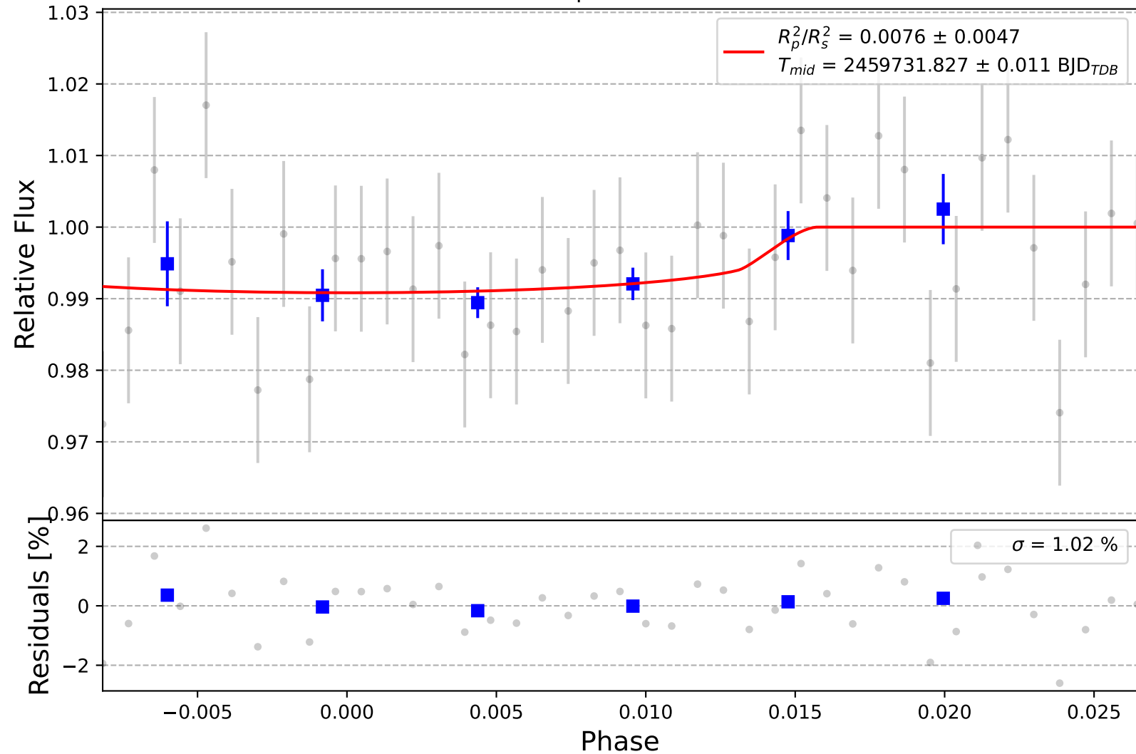
Kepler-553 b
