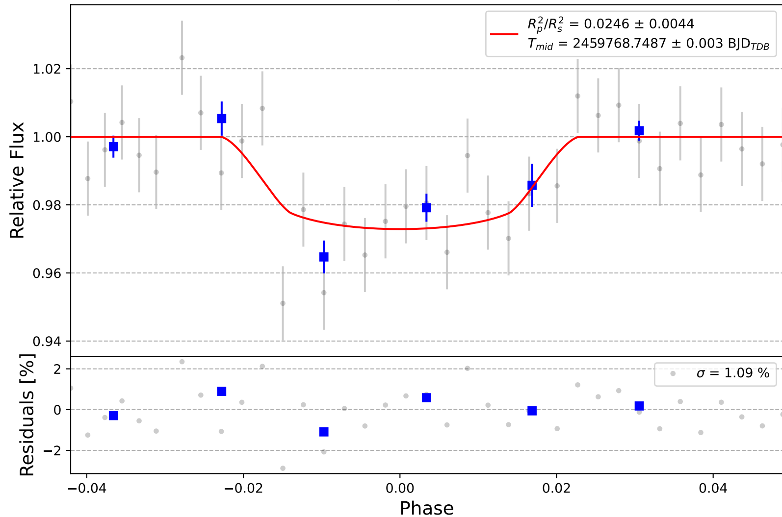
Kepler-686 b
