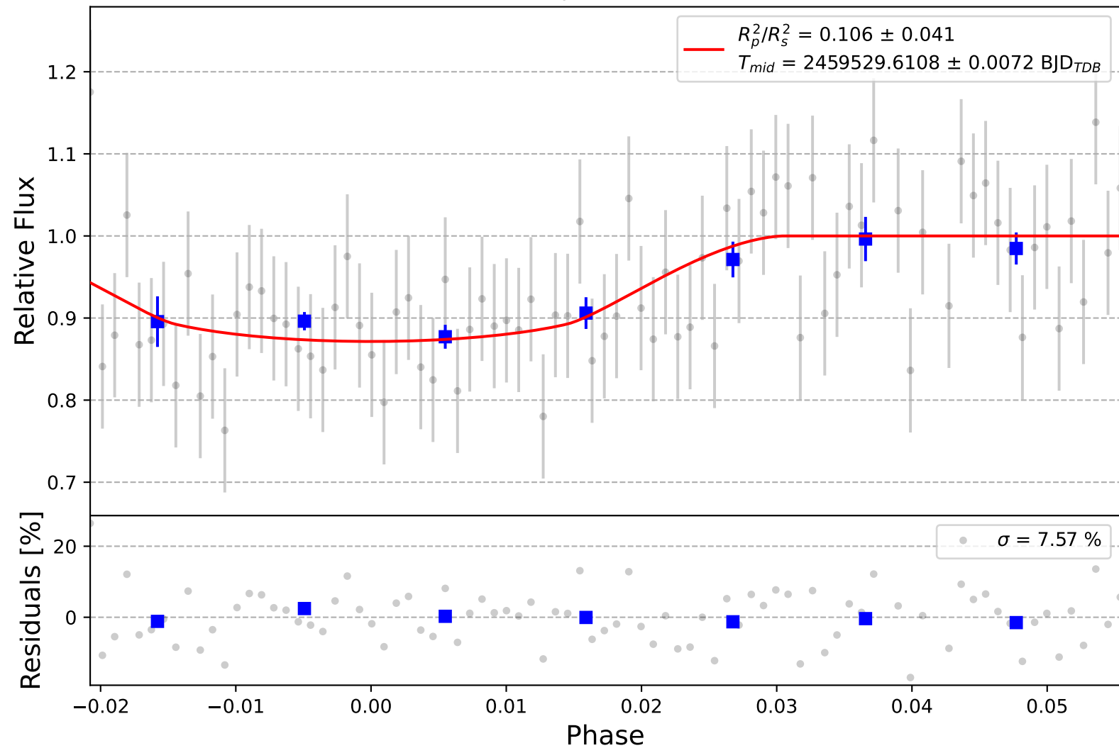
Kepler-785 b
