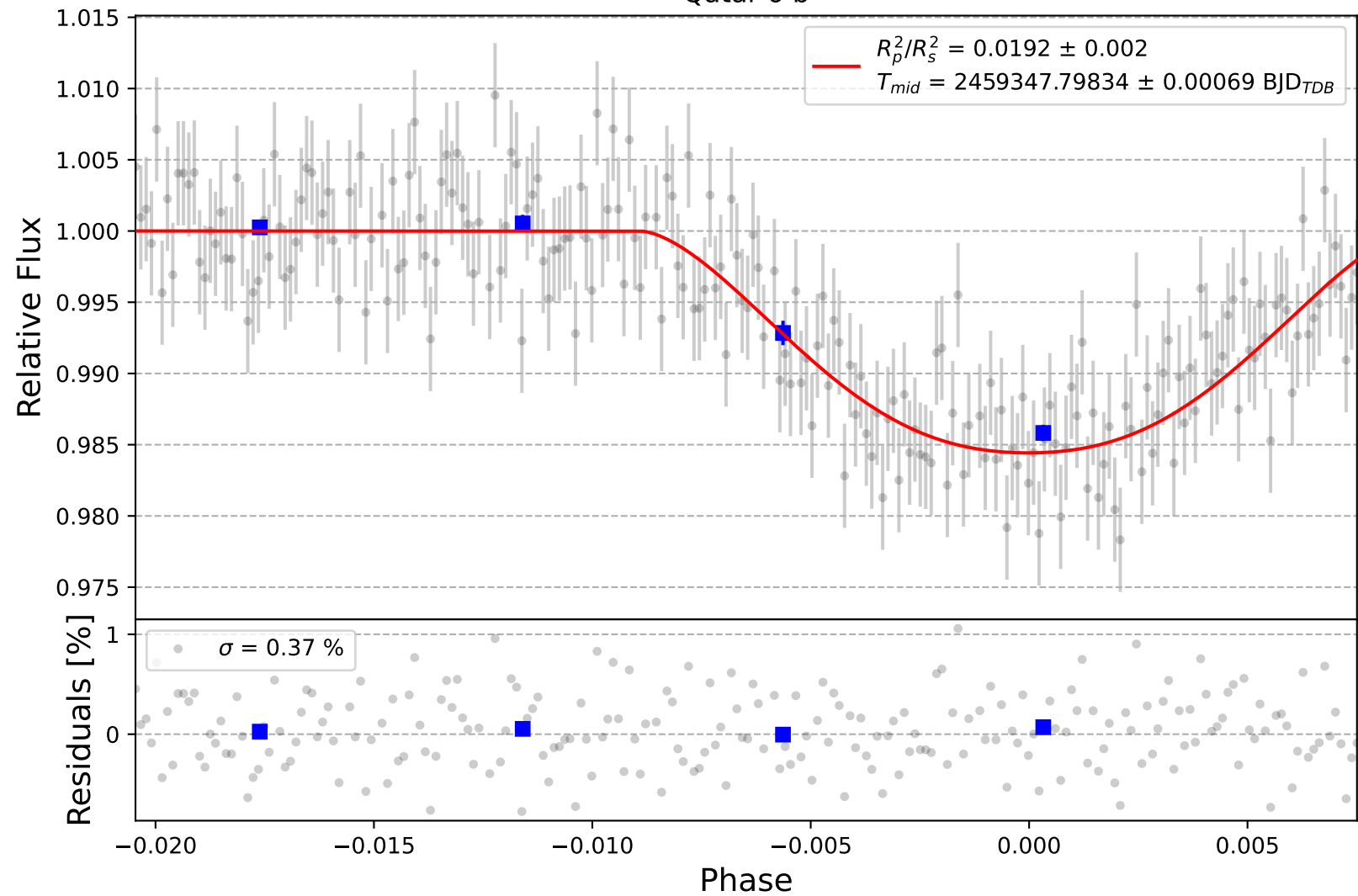
Qatar-6 b
