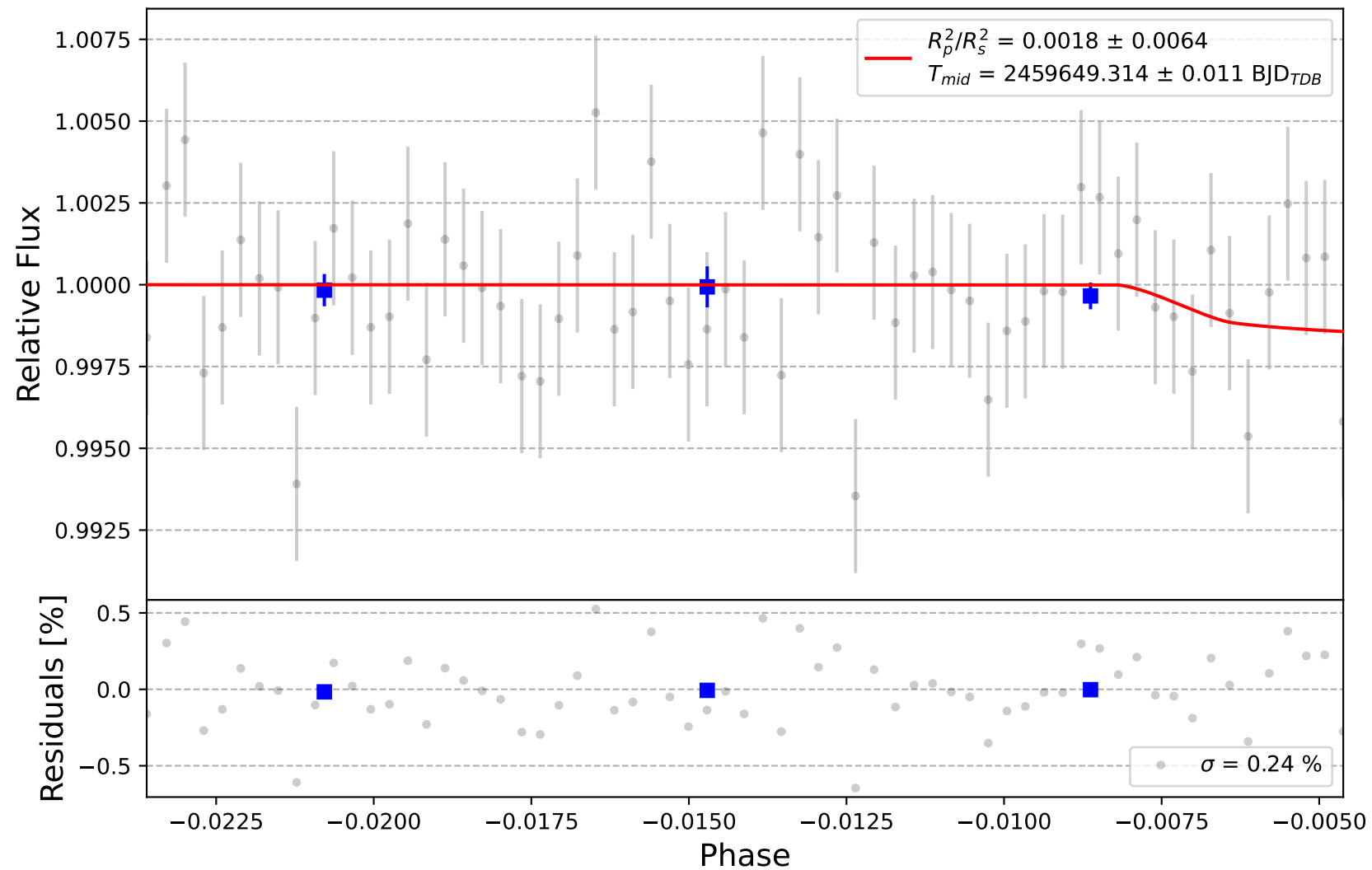
Qatar-6 b
