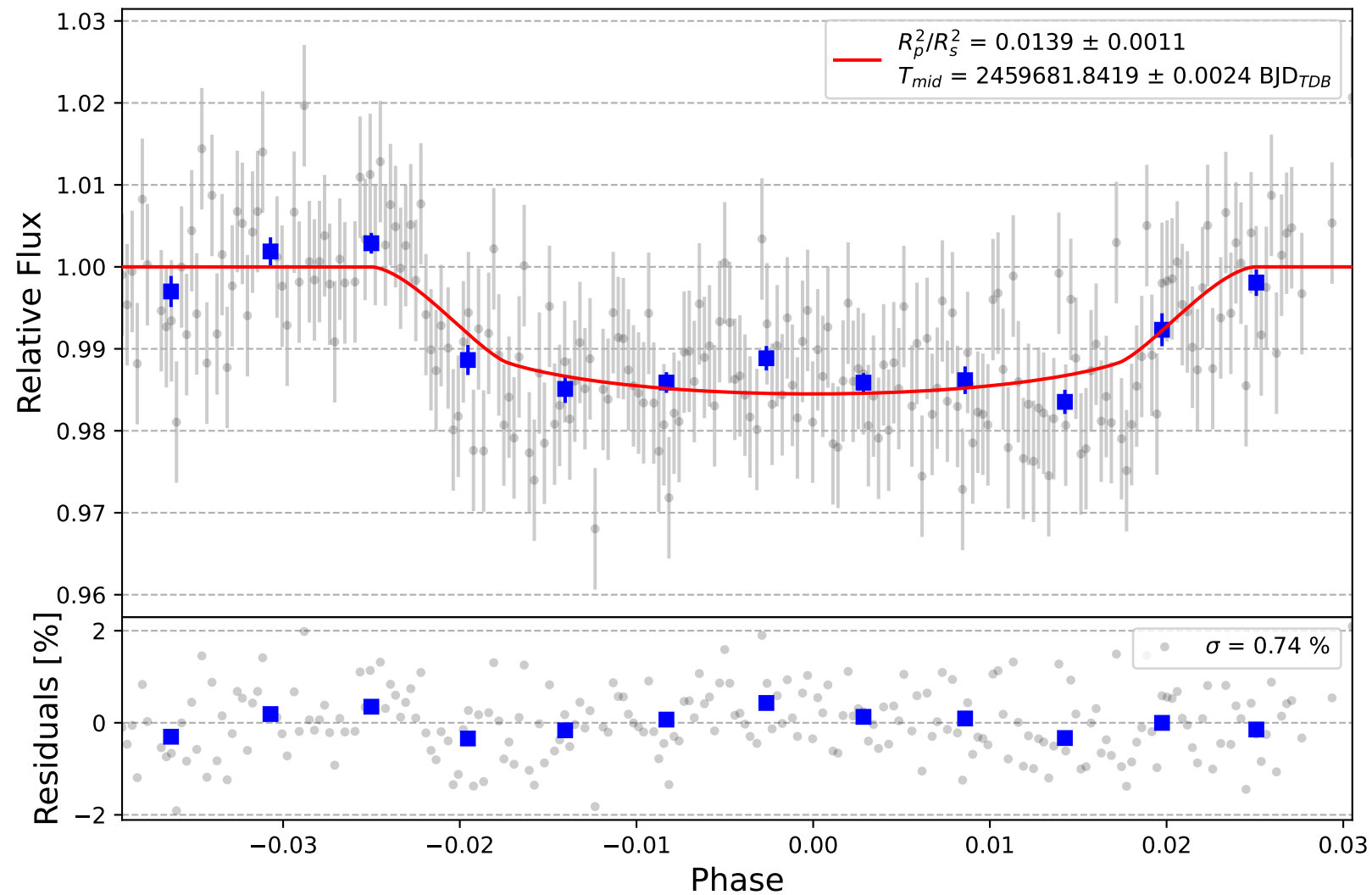
Qatar-8 b
