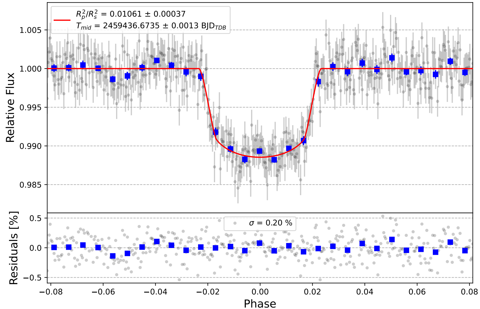
Qatar-8 b
