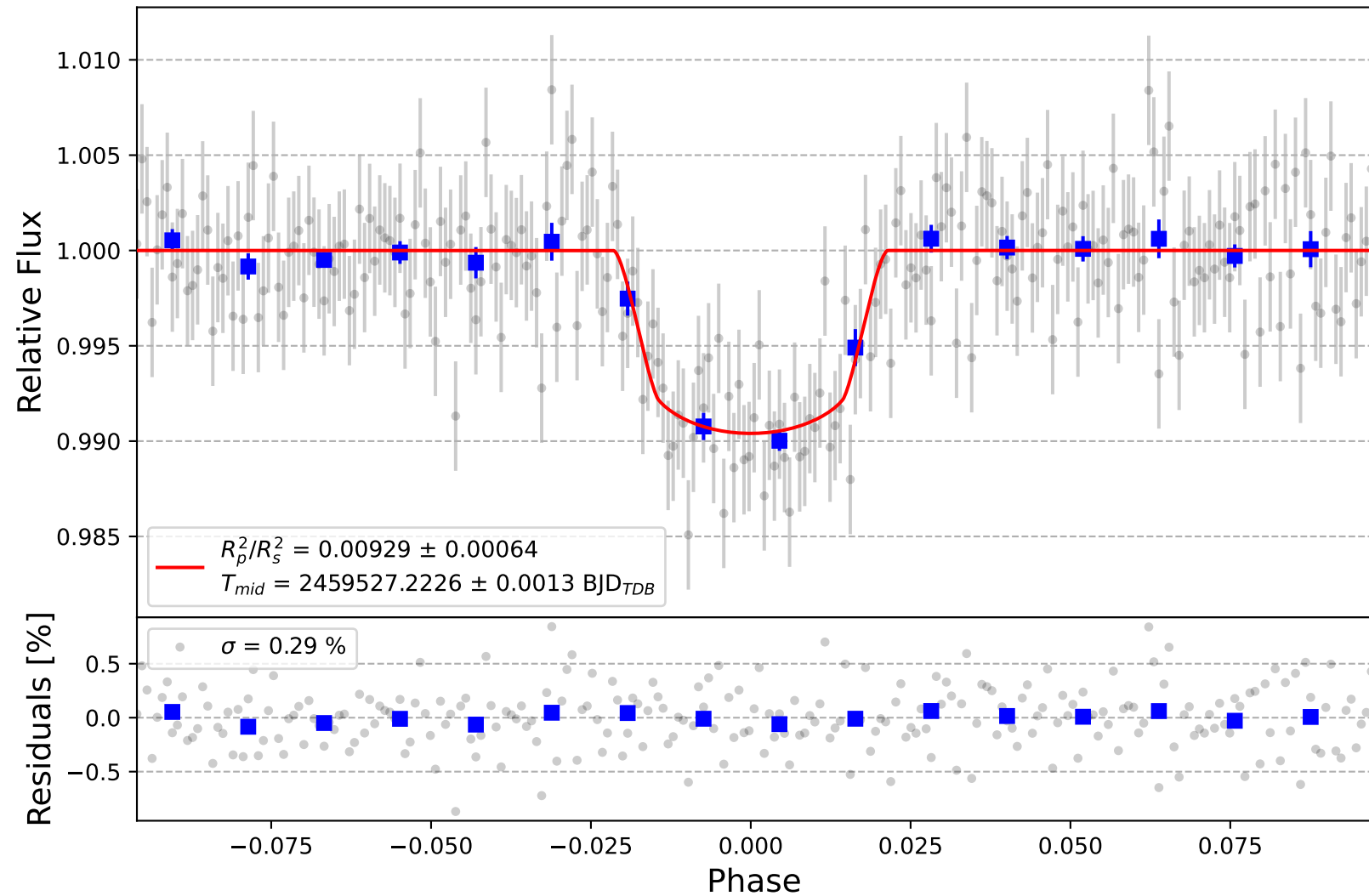
WASP-104 b
