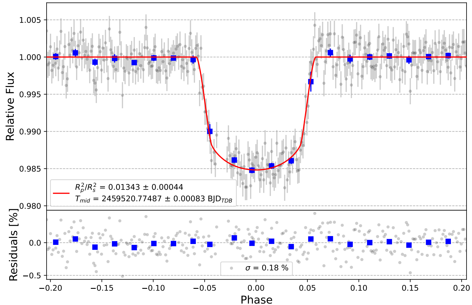
WASP-12 b
