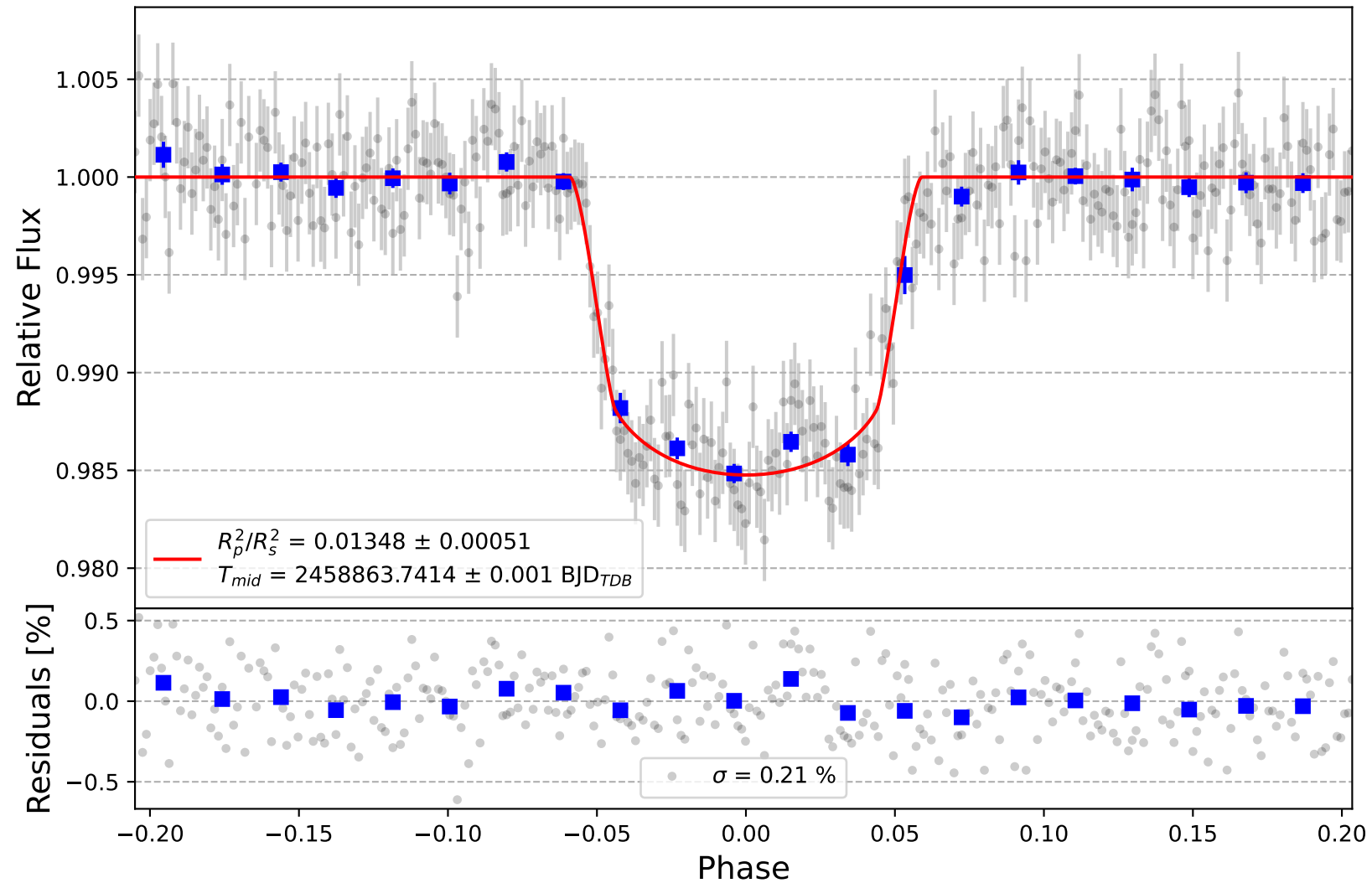
WASP-12 b
