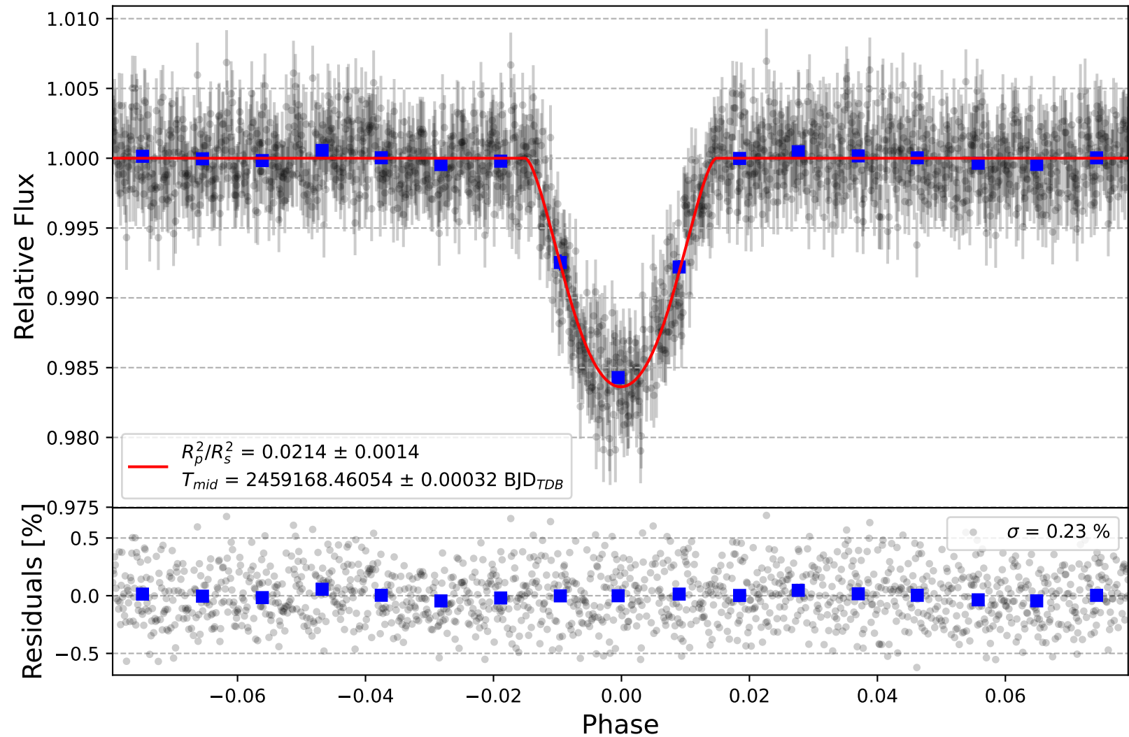
WASP-140 b
