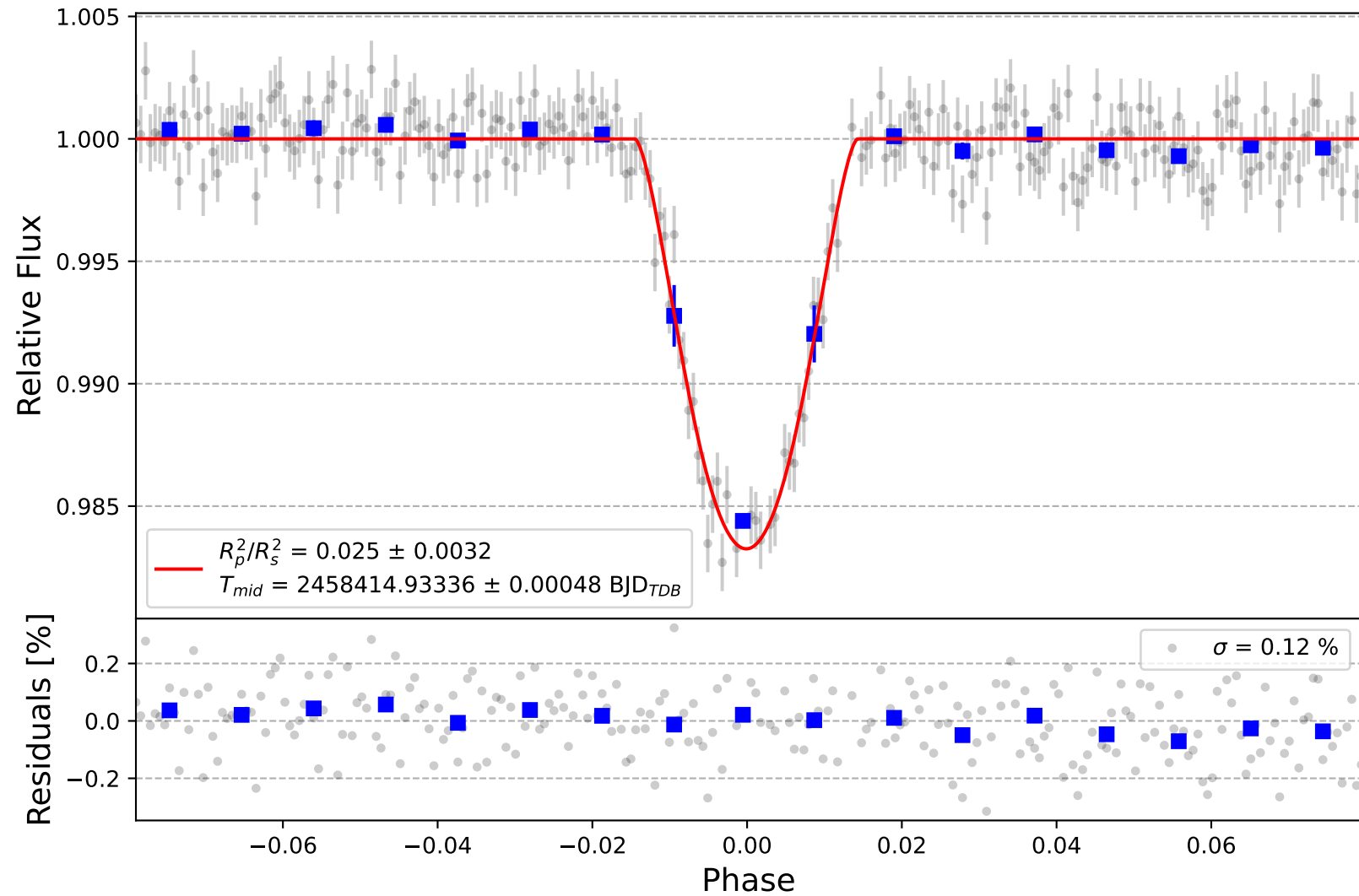
WASP-140 b
