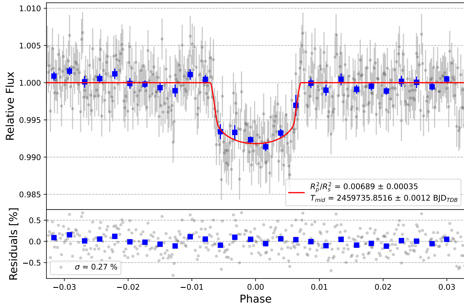
WASP-148 b
