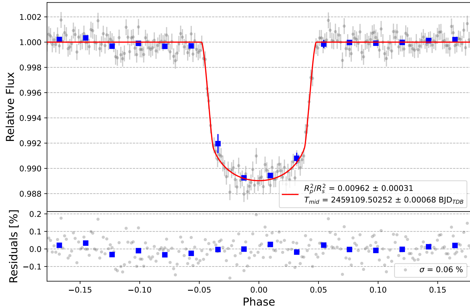
WASP-18 b
