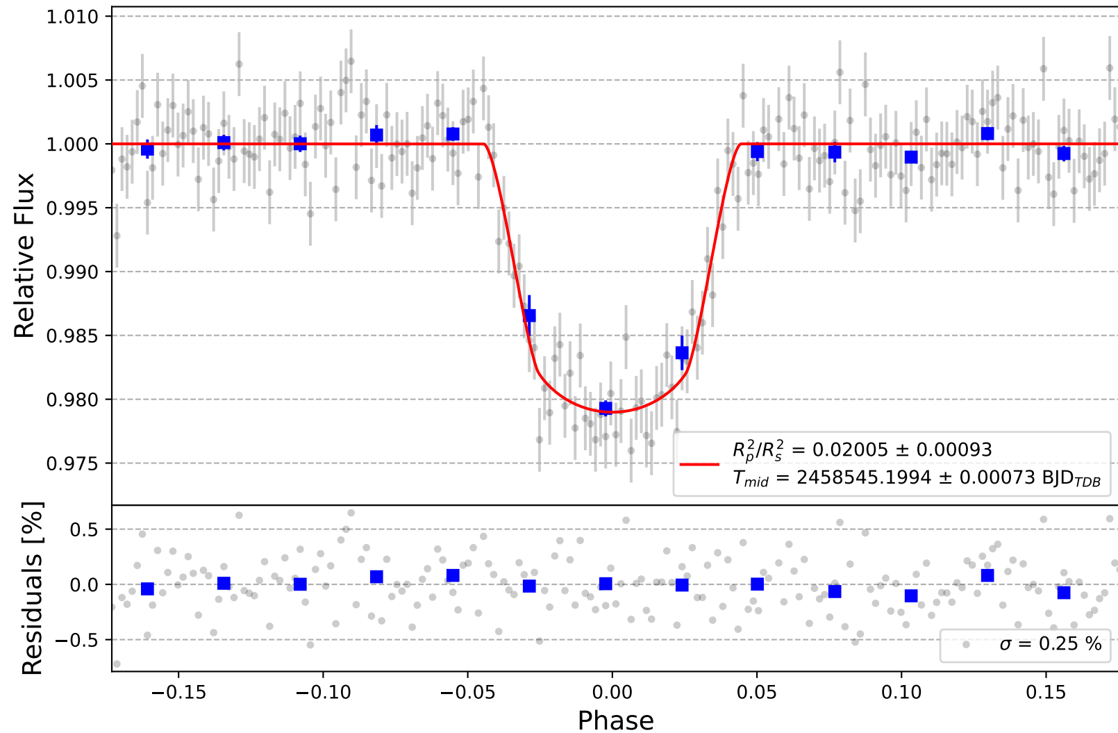
WASP-19 b
