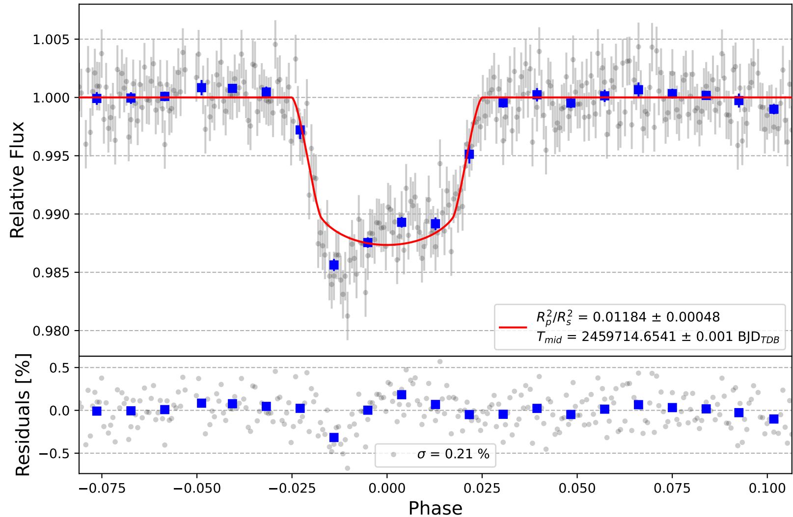
WASP-24 b
