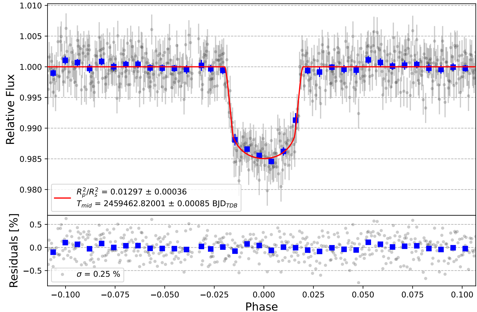
WASP-28 b
