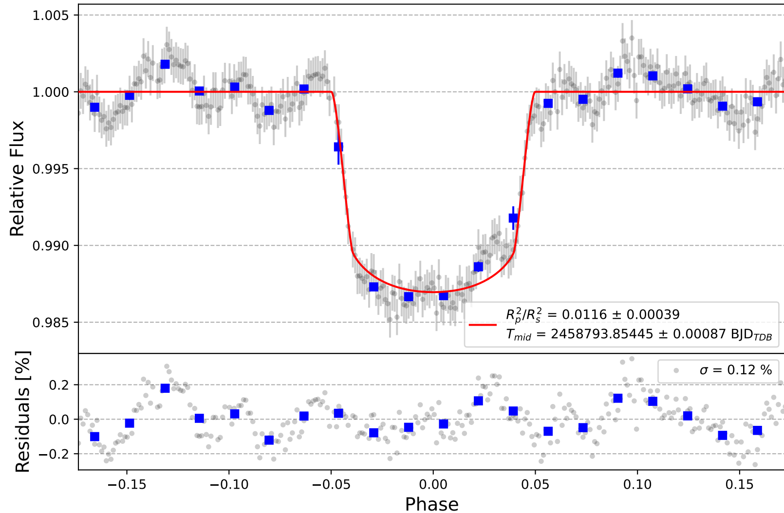
WASP-33 b
