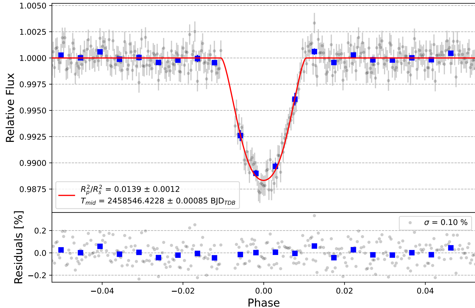
WASP-34 b
