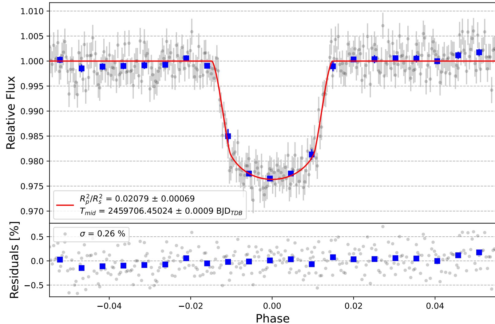
WASP-39 b
