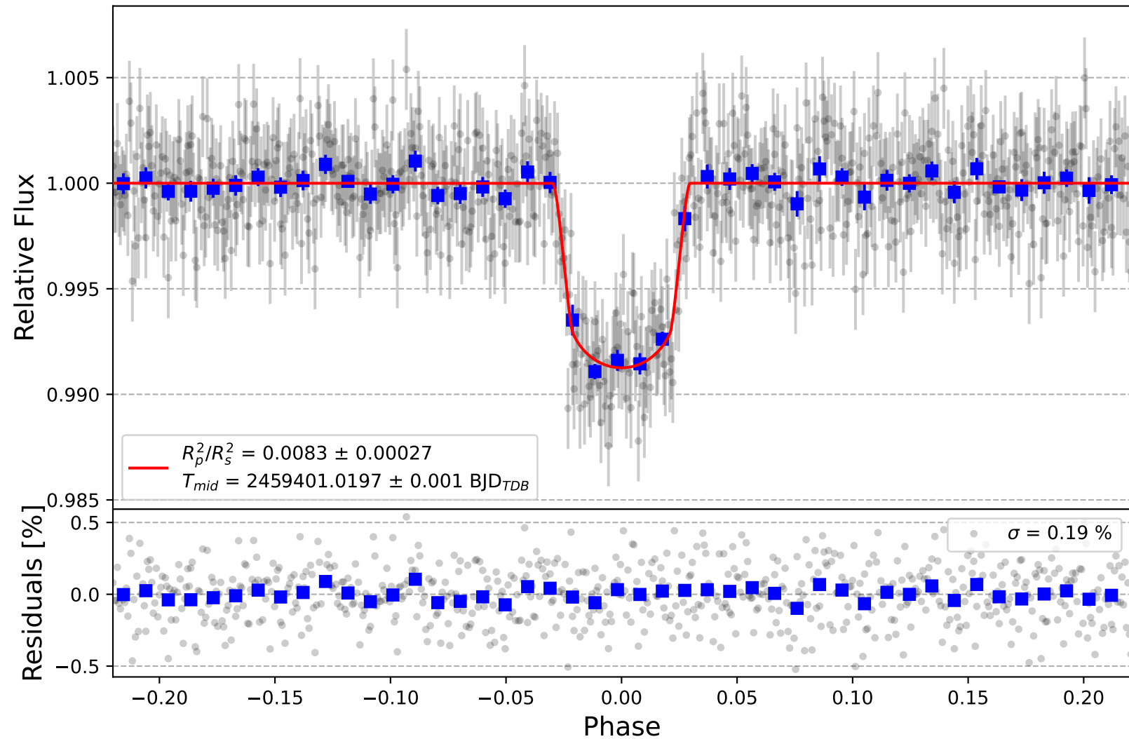
WASP-48 b
