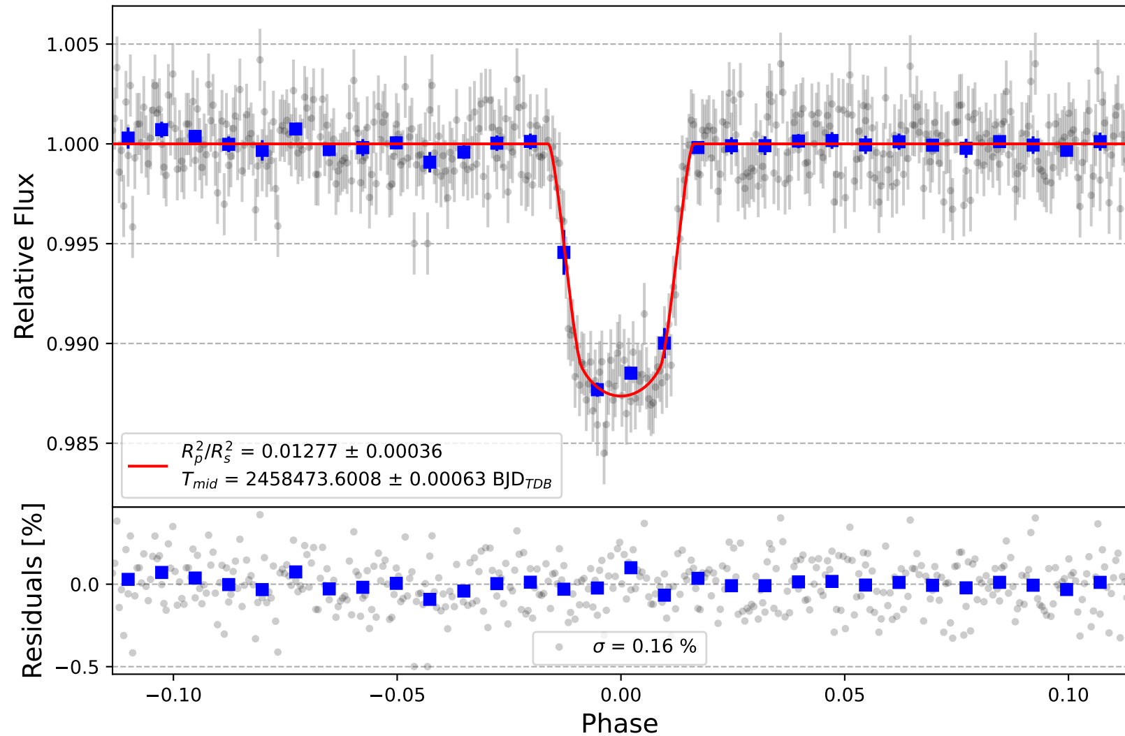
WASP-49 b
