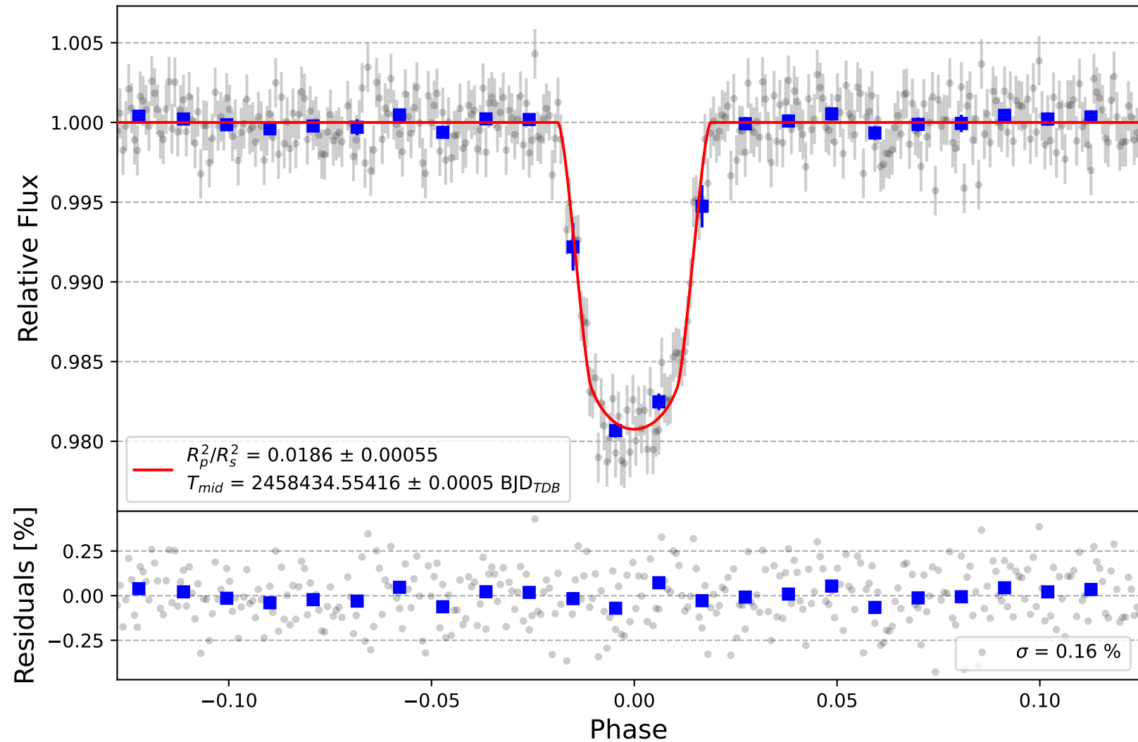
WASP-50 b
