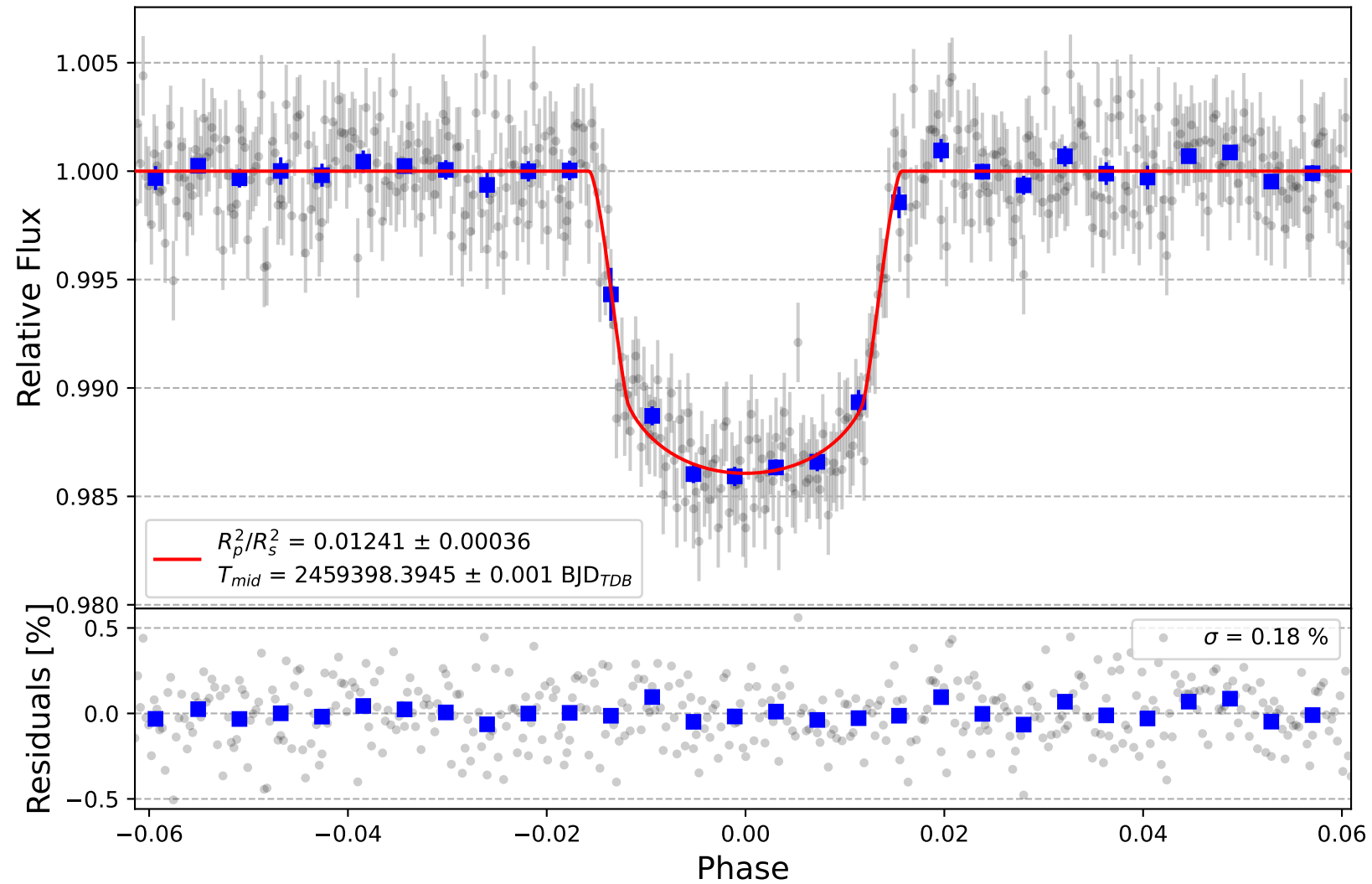
WASP-58 b
