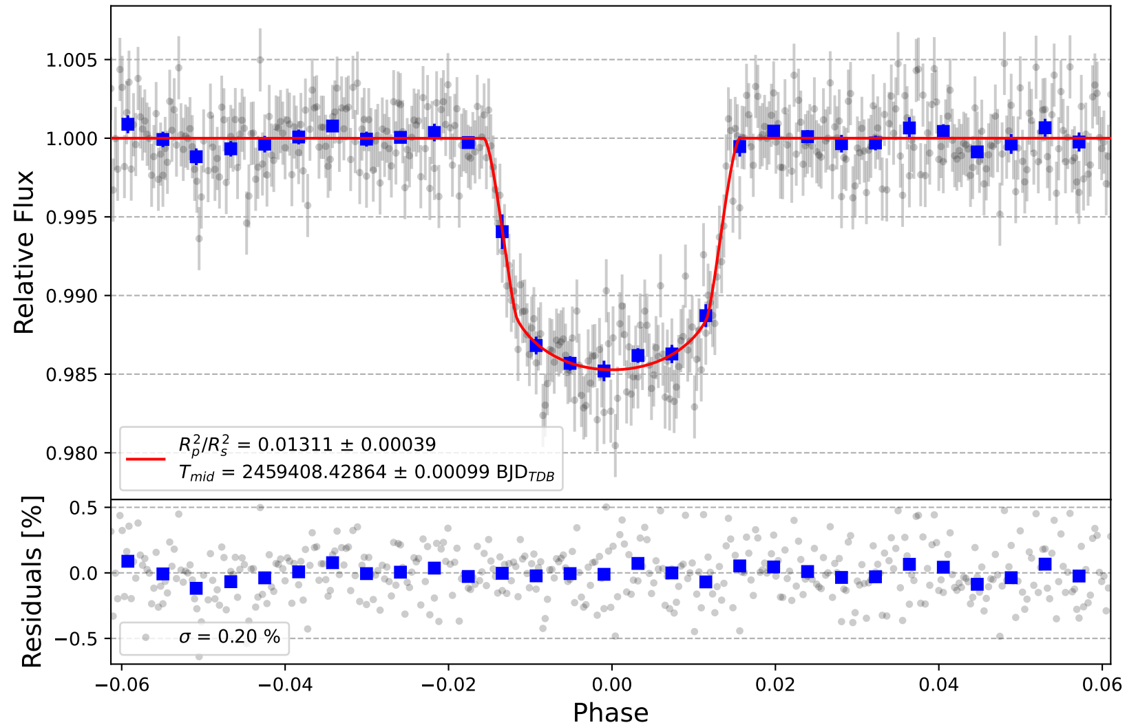
WASP-58 b
