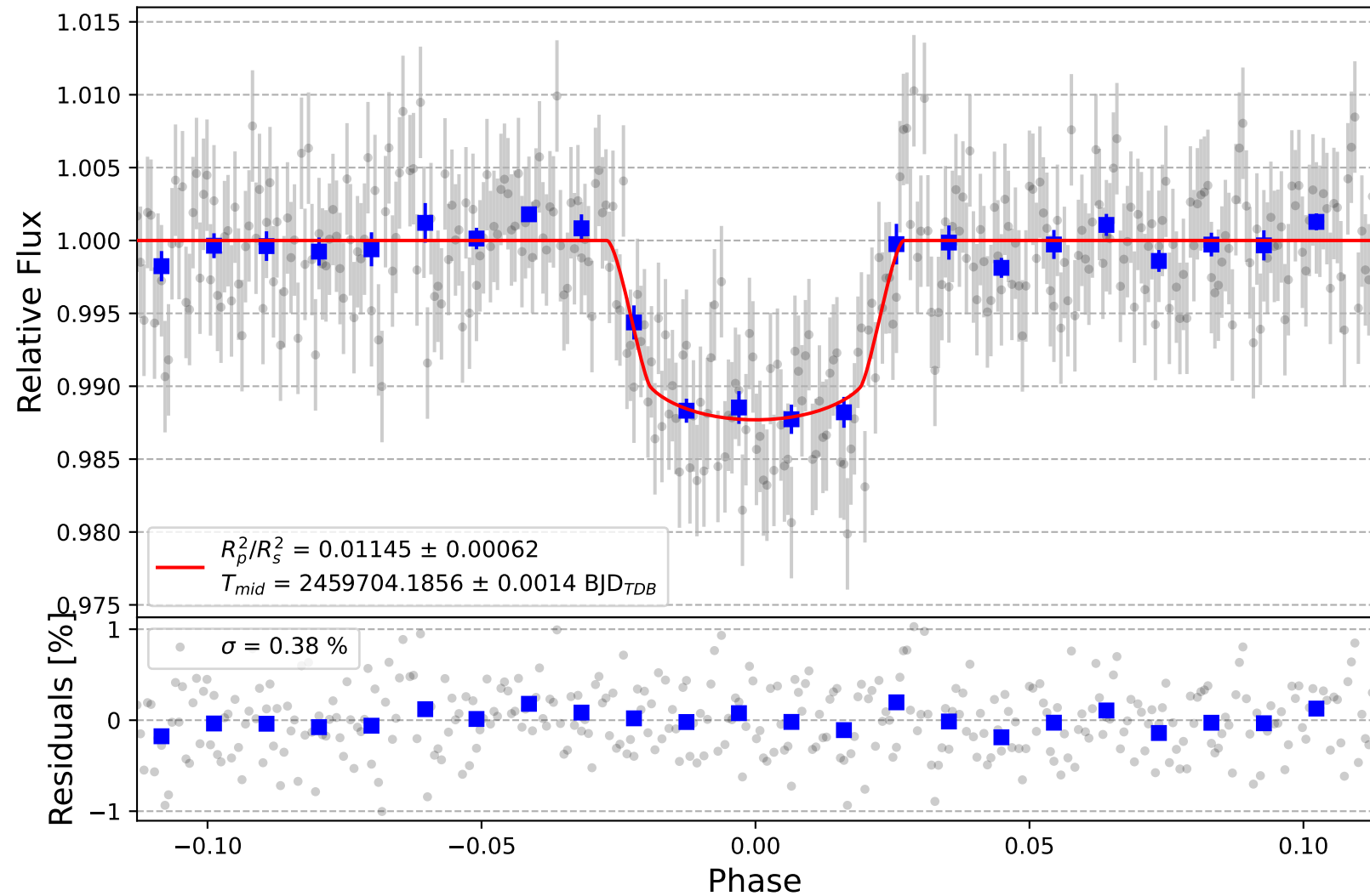
WASP-92 b
